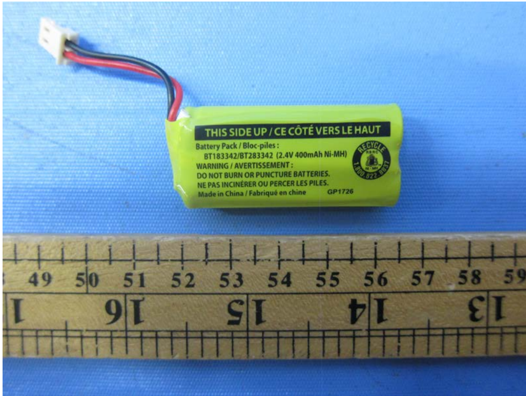
Figure 3 - 2.4V 400mAh GPI Ni-MH rechargeable battery
