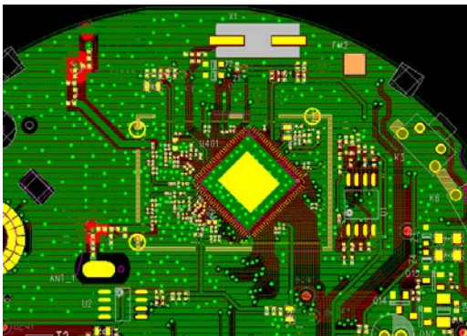
VH6210 BS Mainboard layout
