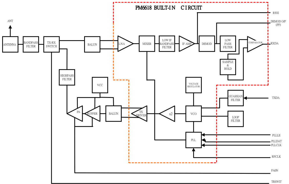
RF BLOCK DIAGRAM OF Base (INFINEON PM6618)
