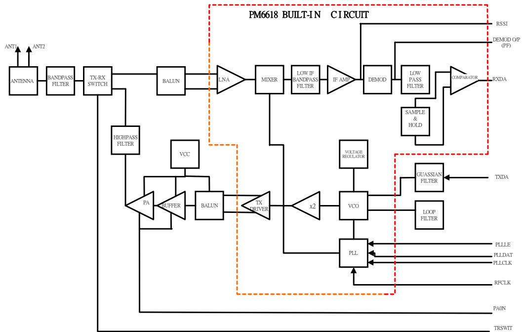
RF BLOCK DIAGRAM OF HANDSET (INFINEON PM6618)
