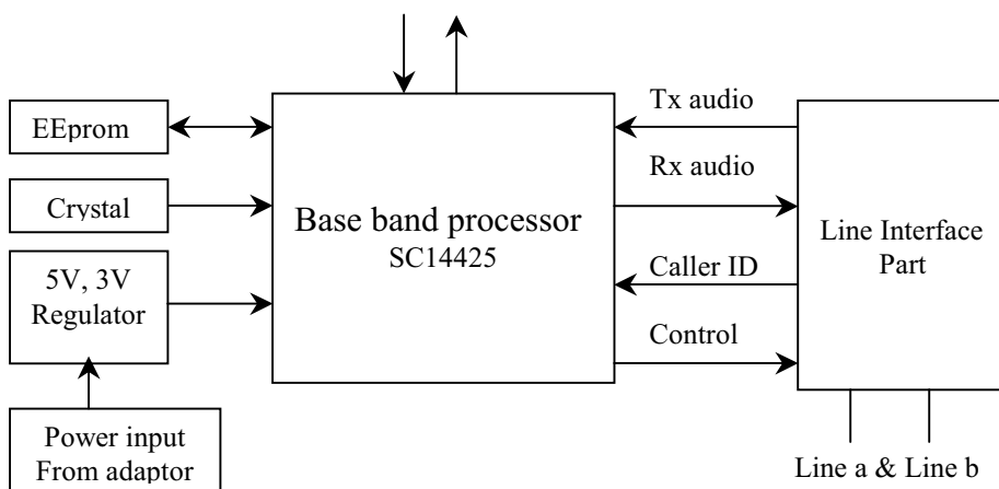
Base block diagram
