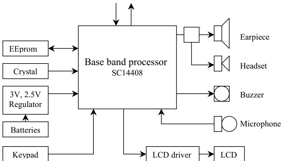
Handset block diagram
