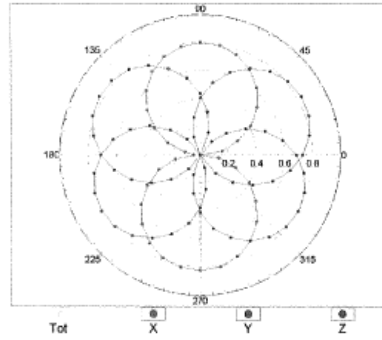
f=600 MHz,TEM
