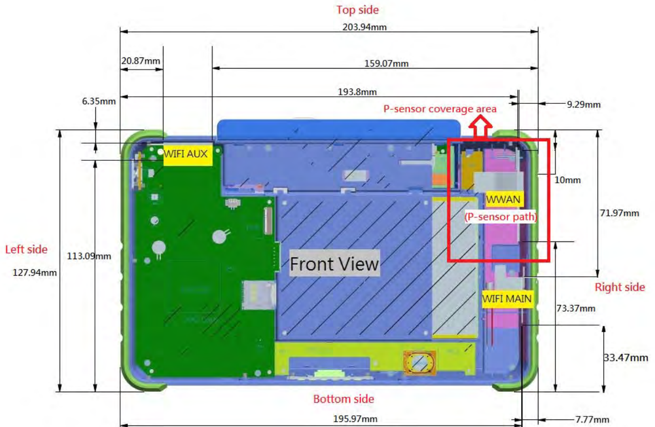
Fig.10 Antenna position of EUT (Front view)
