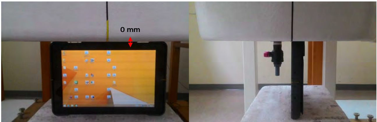
Fig.4 EUT Top side to flat phantom
