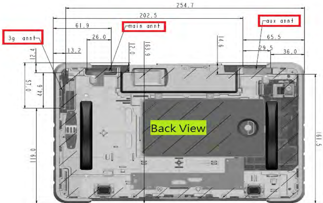
Fig.7 Back view of EUT
