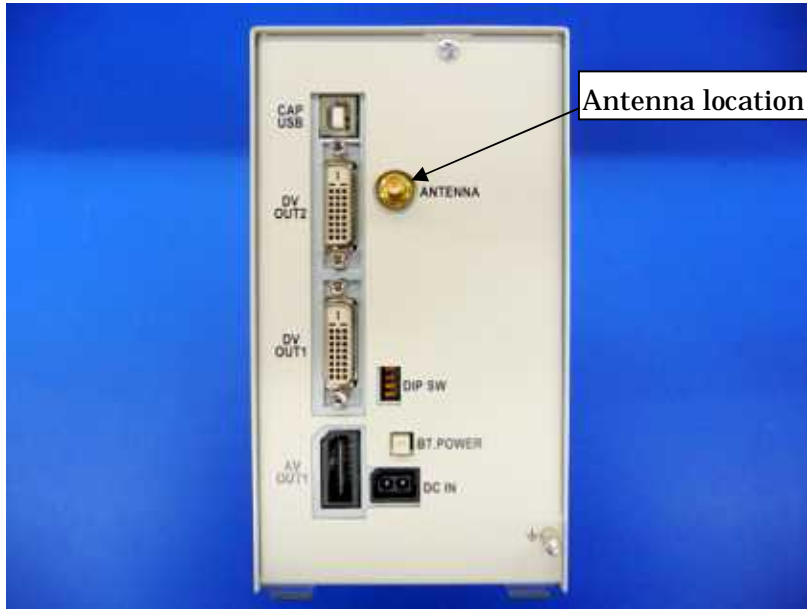
Back view (Capture)
