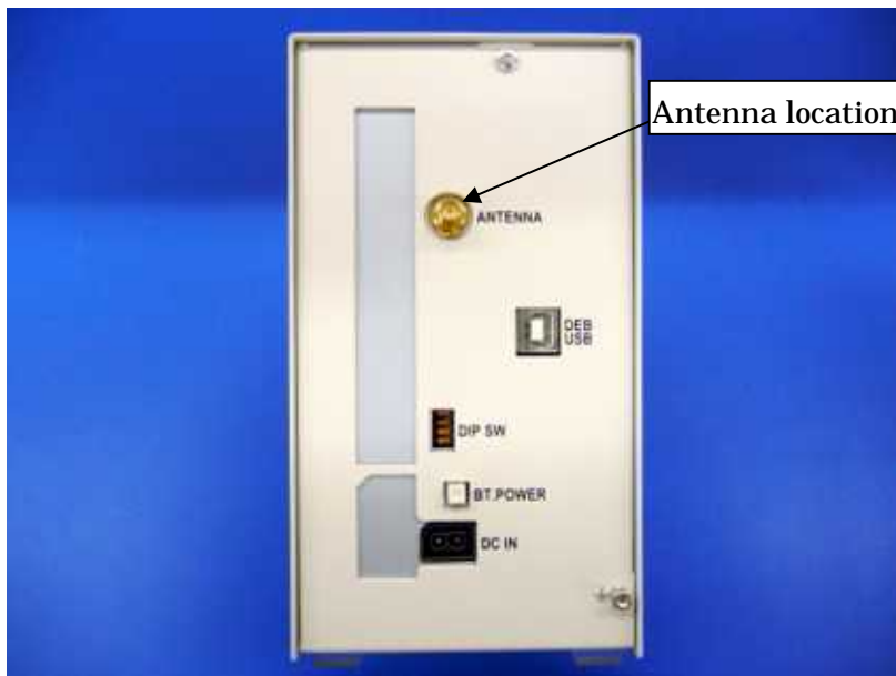
Back view (Debugger)
