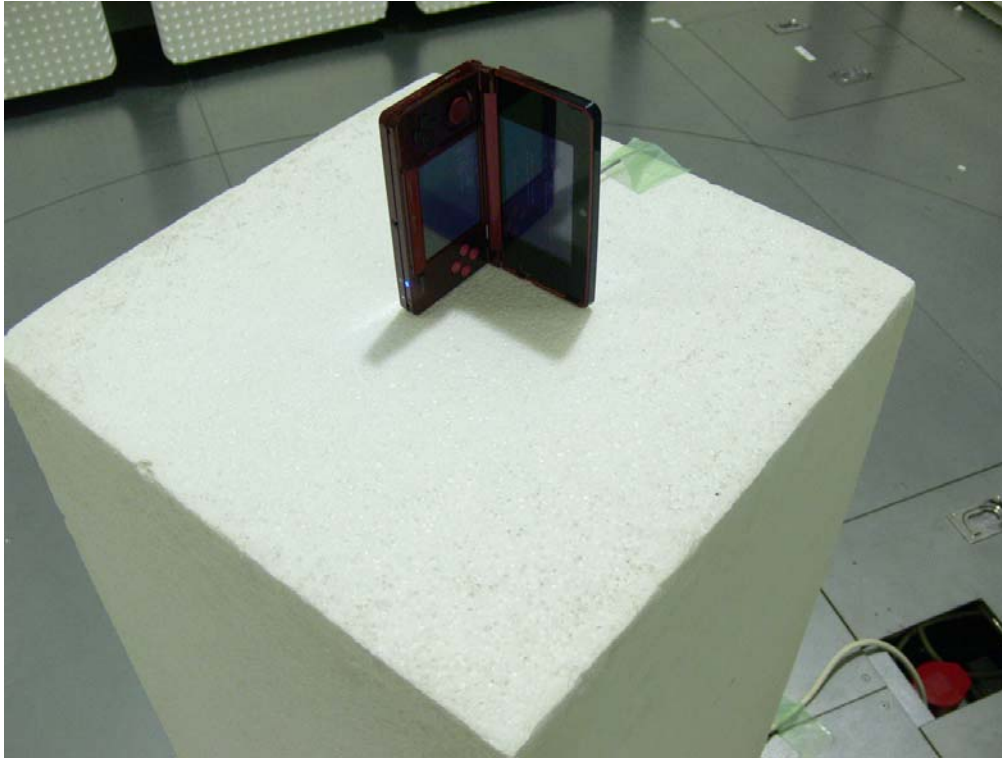
Photograph 4: Set-up for Radiated Emission, EUT Configuration Y-Axis (Movable antenna)
