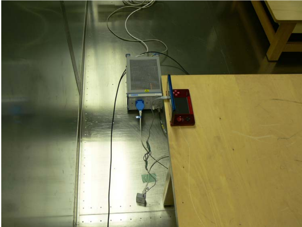
Photograph 2: Set-up for AC Mains Conducted Emission of Transmitter and Receiver, Rear View
