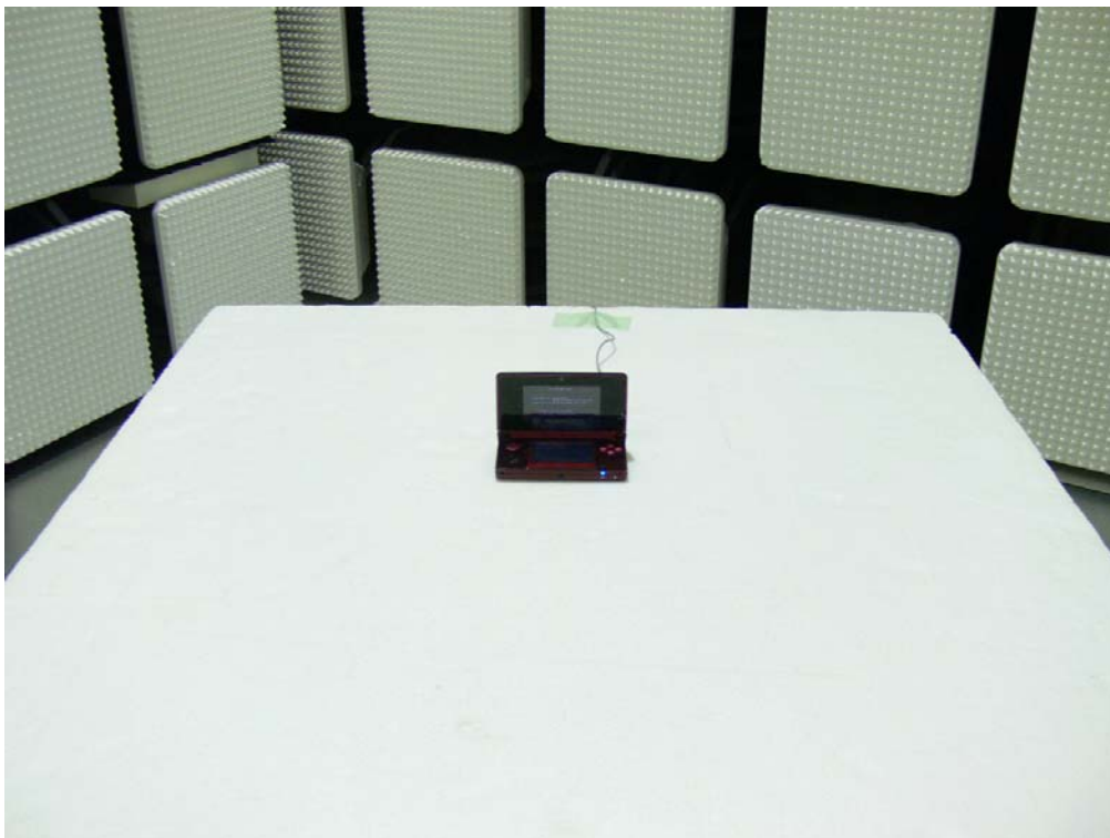
Photograph 3: Set-up for Radiated Emission, EUT Configuration X-Axis (Movable antenna)
