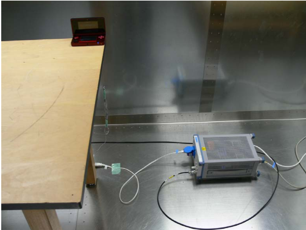
Photograph 1: Set-up for AC Mains Conducted Emission of Transmitter and Receiver, Front View
