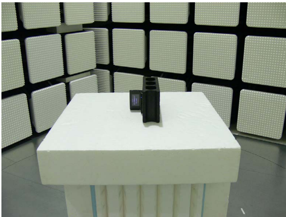
Photograph 5: Set-up for Radiated Emission, EUT Configuration Z-Axis (Movable antenna)
