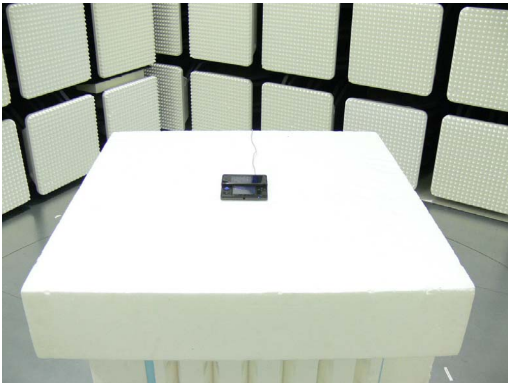
Photograph 3: Set-up for Radiated Emission, EUT Configuration X/Y-Axis (Movable antenna)
