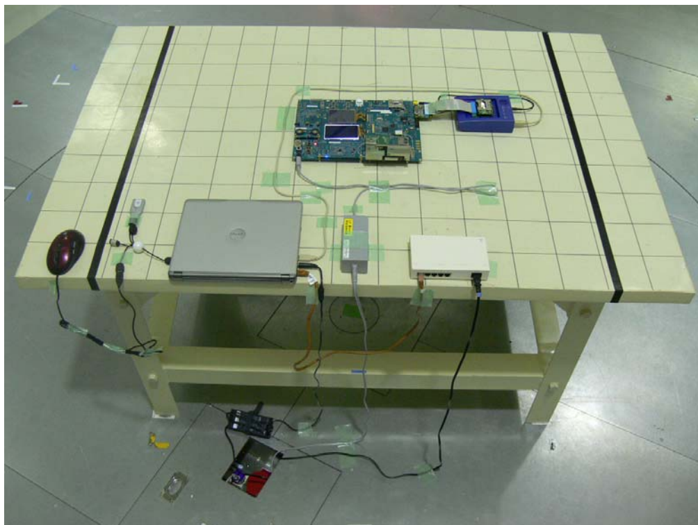
Photograph 9: Set-up for Radiated Emission of Transmitter, Rear View
