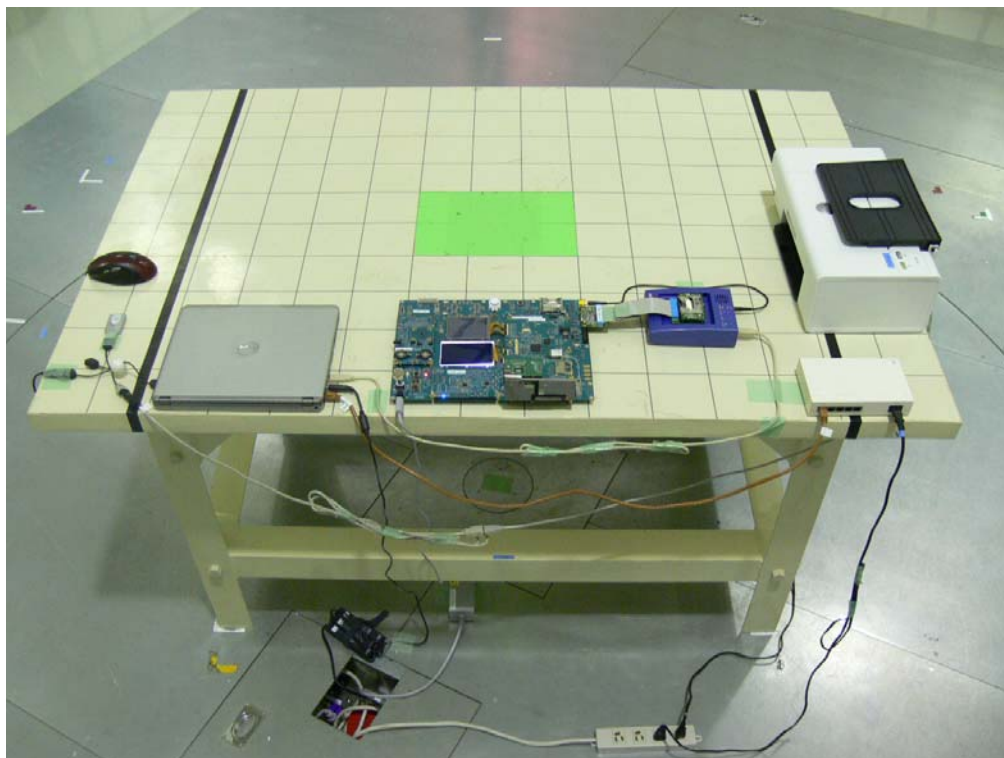
Photograph 11: Set-up for Radiated Emission of Receiver, Rear View
