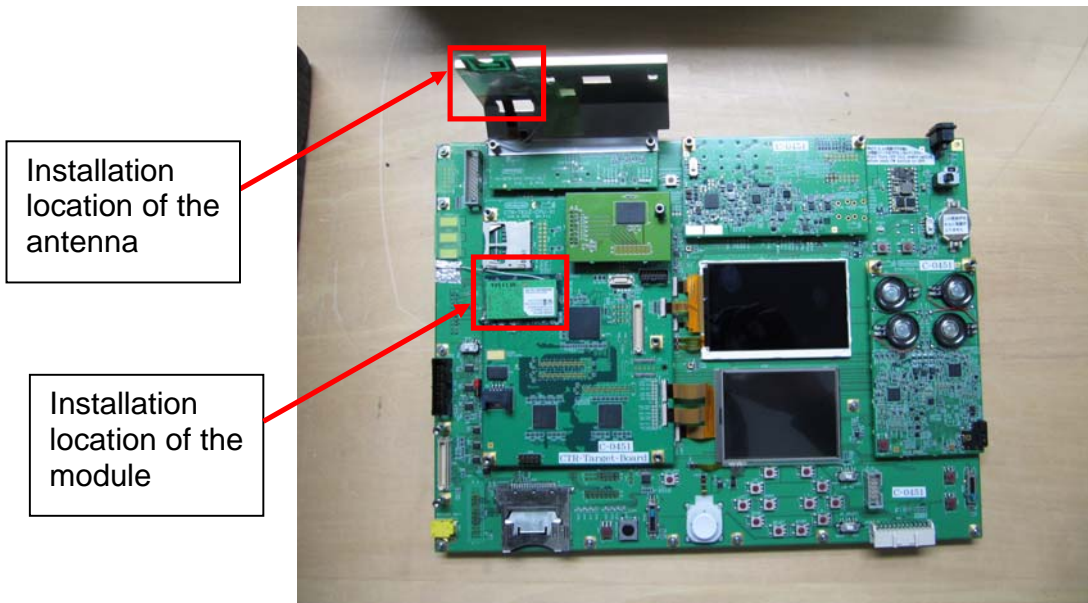
Top view (Nintendo DS CTR TARGET BOARD / assembled completely)
