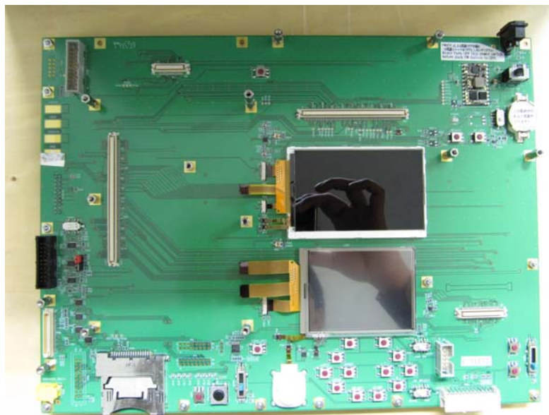
Top view (Nintendo DS CTR TARGET BOARD / mother part)
