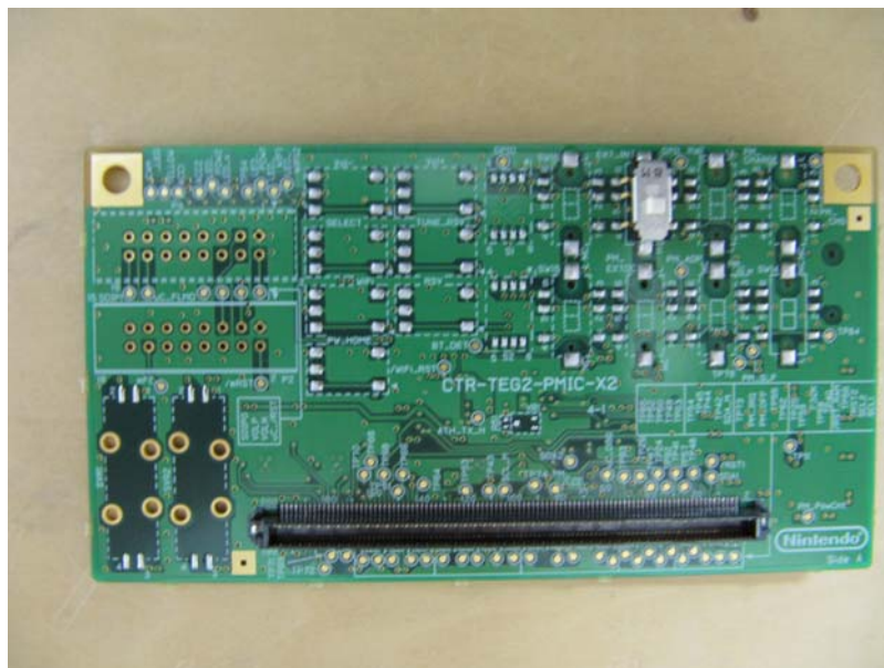
Bottom view (Nintendo DS CTR TARGET BOARD / Power Management IC part)
