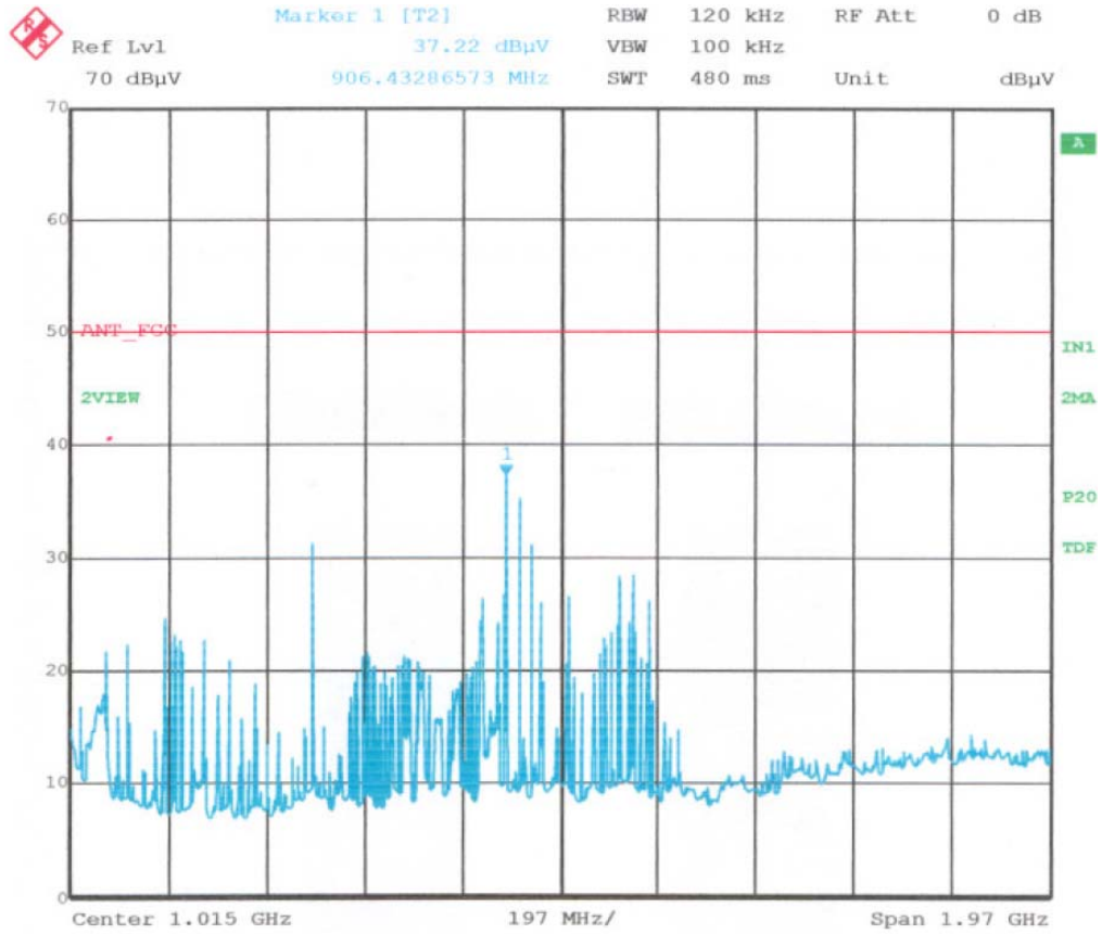
< Fig 6. Antenna power conduction result >
