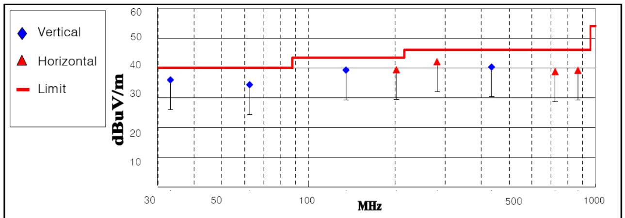
< Fig 5. Radiated emission result >
