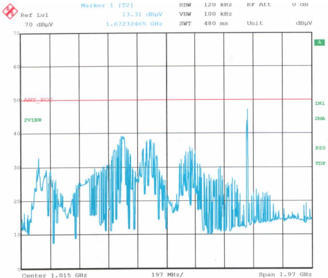
< Fig 7. Antenna power conduction result >
