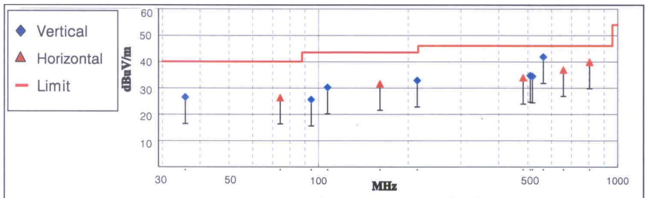
< Fig 6-2. Radiated emission result >
