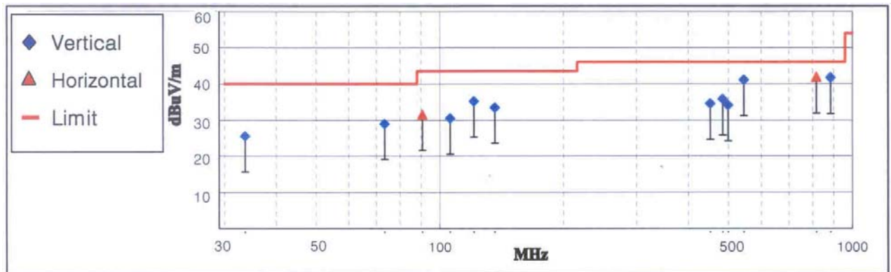
< Fig 6-2. Radiated emission result >
