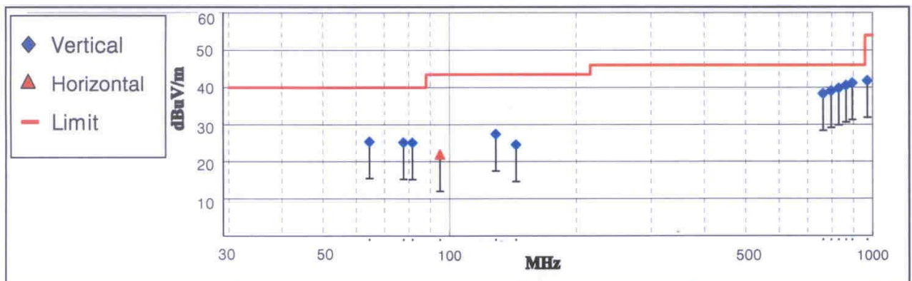
< Fig 6-2. Radiated emission result >
