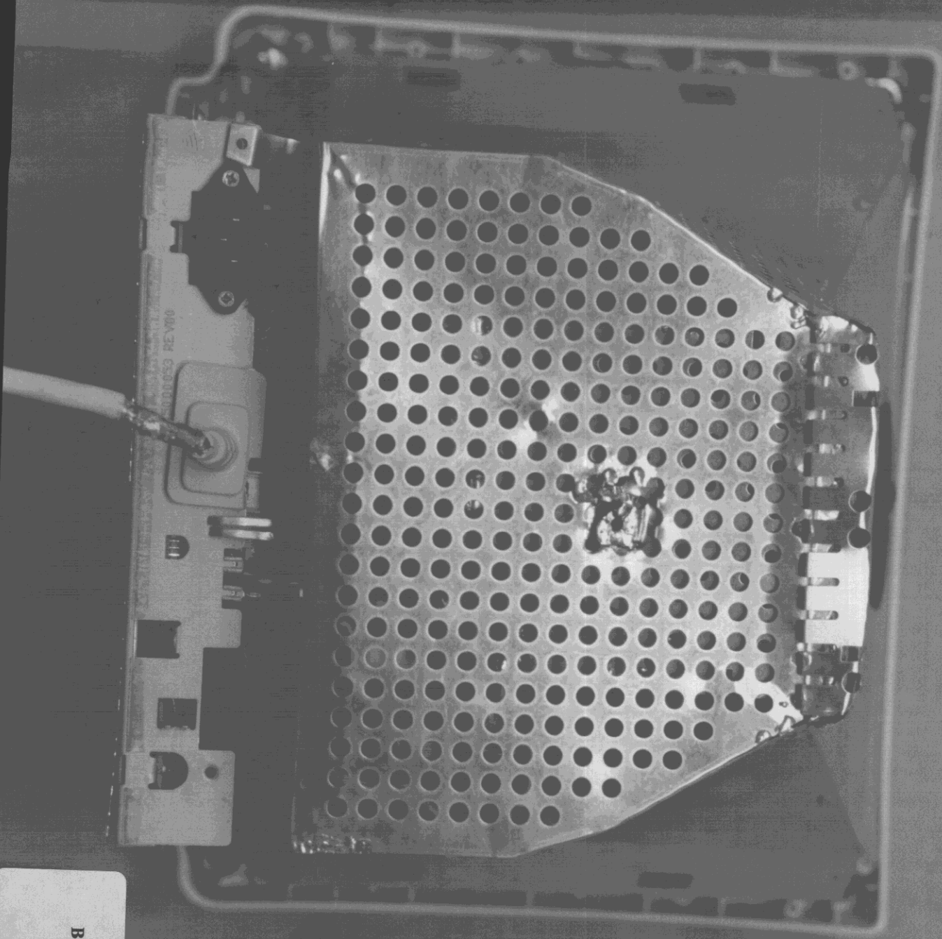
Figure 6 Back of Monitor, with Shield
