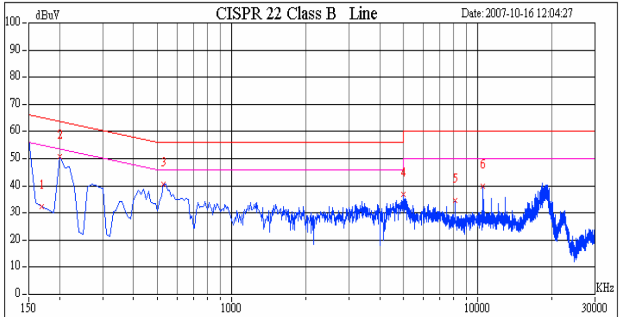
Conducted emissions (Line 1)
