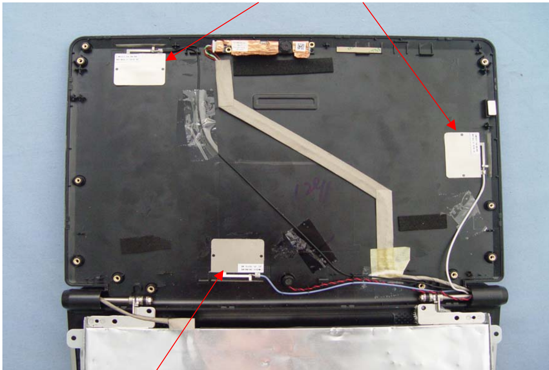
Bluetooth Antenna
