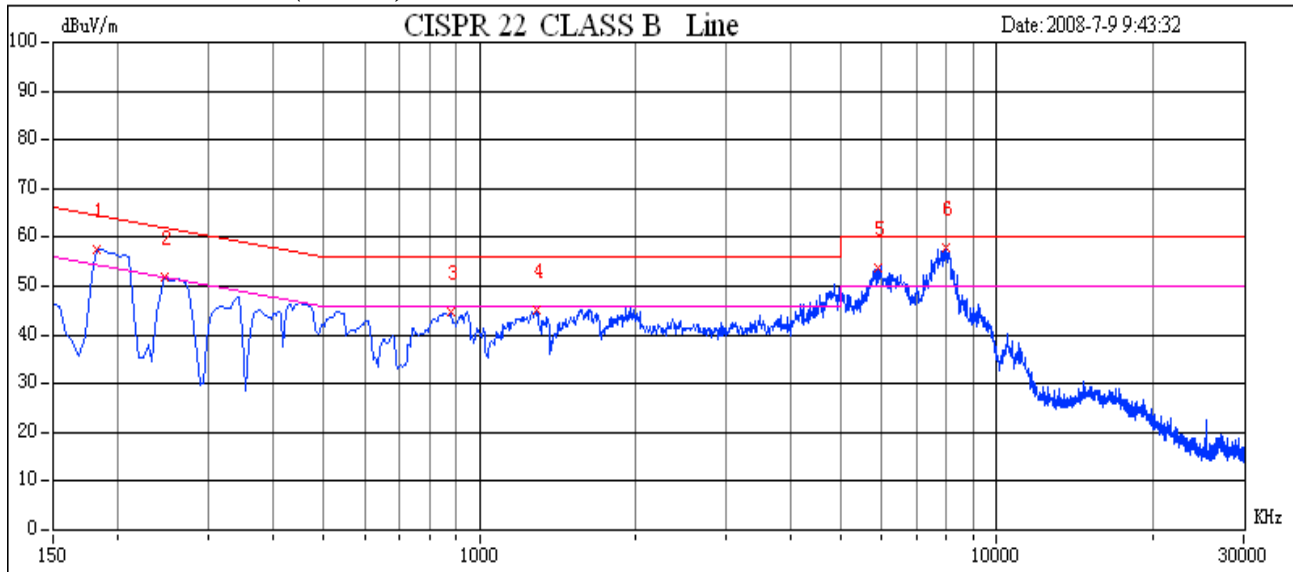
Conducted emissions (Line 1)
