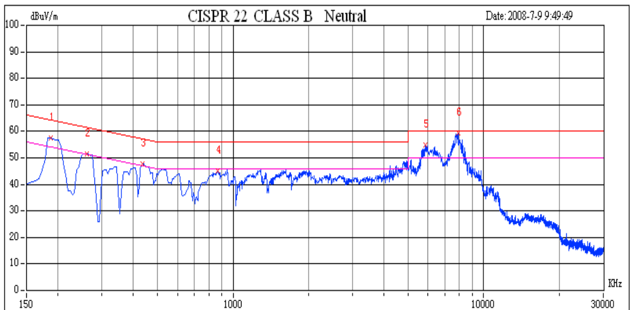
Conducted emissions (Line 2)
