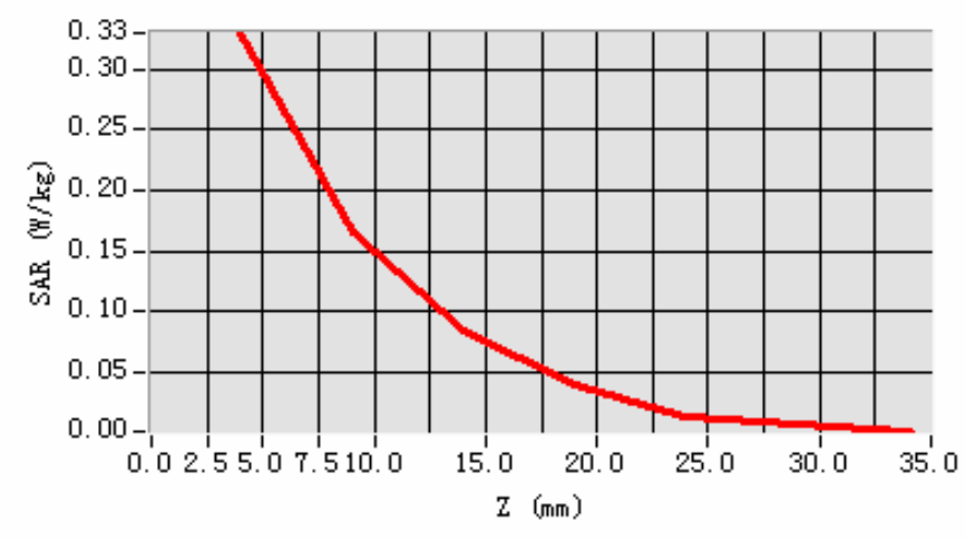
SAR, Z Axis Scan (X = 0, Y = -7)
