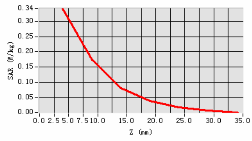
SAR, Z Axis Scan (X = 0, Y = -5)
