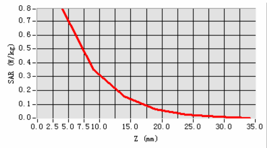
SAR, Z Axis Scan (X = -2, Y = -1)
