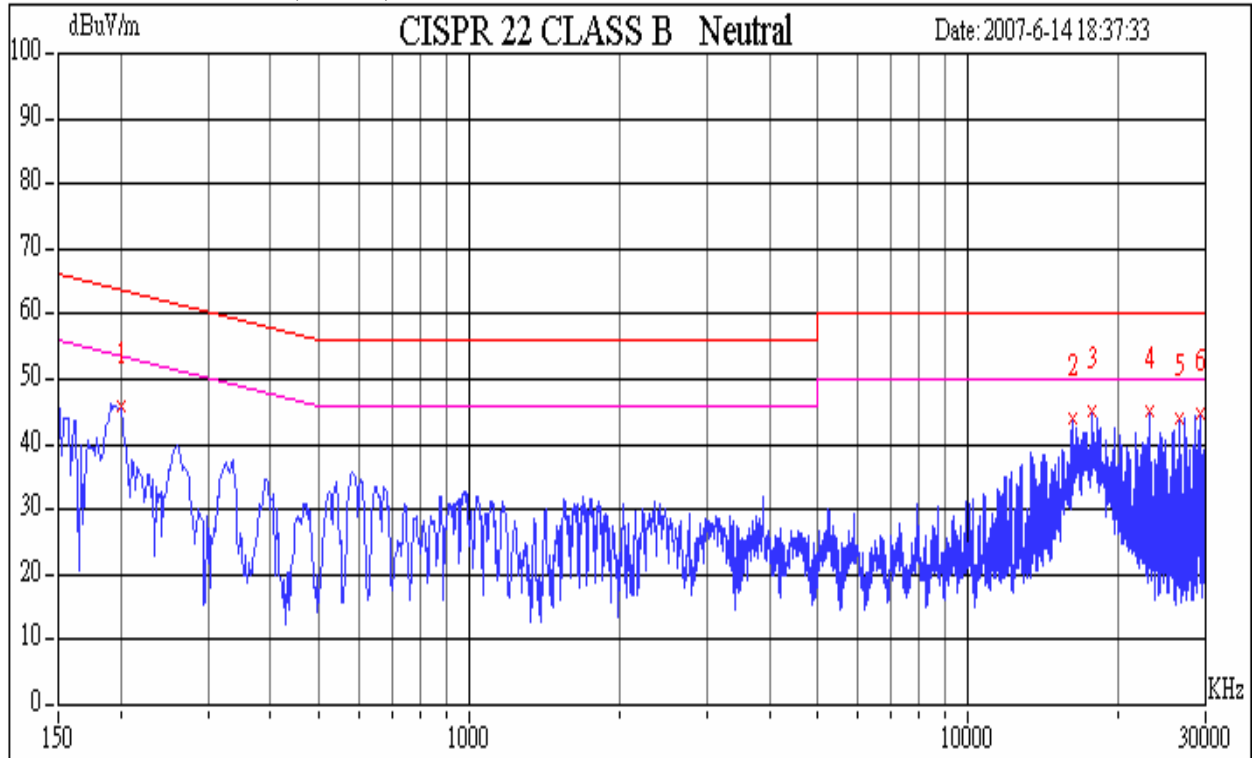
Conducted emissions (Line 2)
