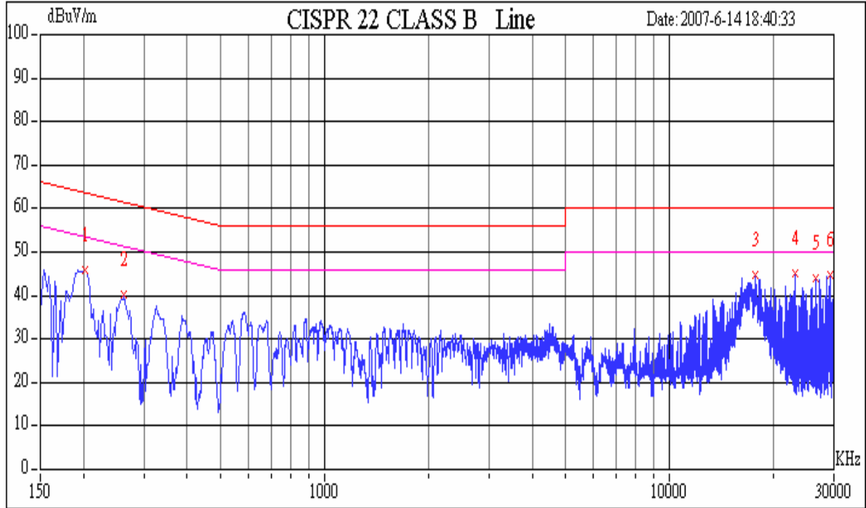
Conducted emissions (Line 1)
