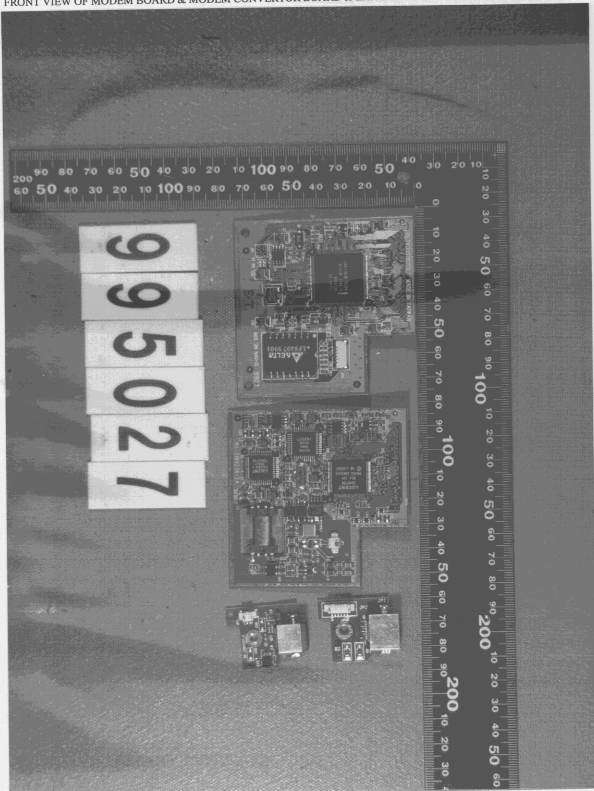
36. FRONT VIEW OF MODEM BOARD & MODEM CONVERTOR BOARD & LAN BOARD & LAN CONVERTOR BOARD
