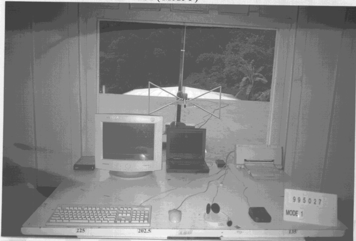
14. BACK VIEW OF RADIATED TEST ( Mode 1 )
