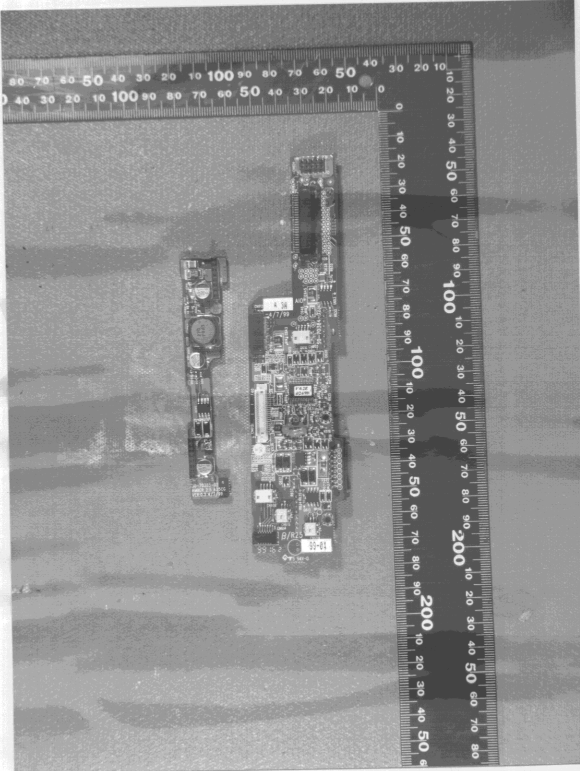
COMPONENT SIDE OF I/O BOARD, DC TO DC BOARD
