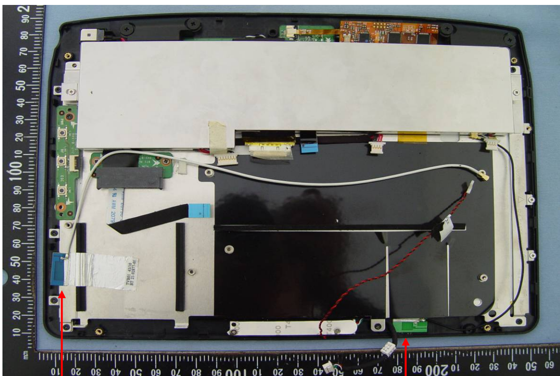
BT Antenna
