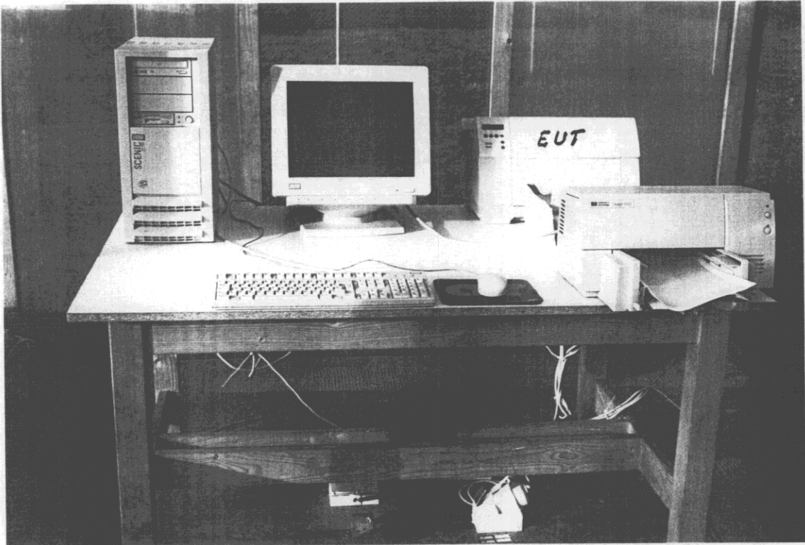
Open field test configuration
