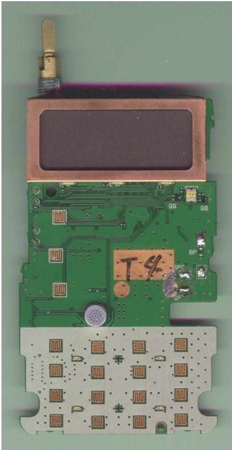
FIGURE 20: Top of CPU Board
