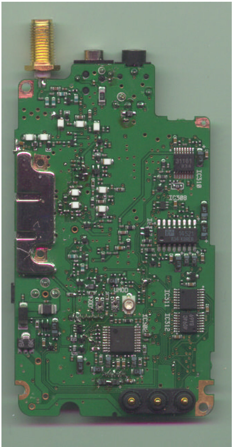
FIGURE 21: Bottom of Main Board
