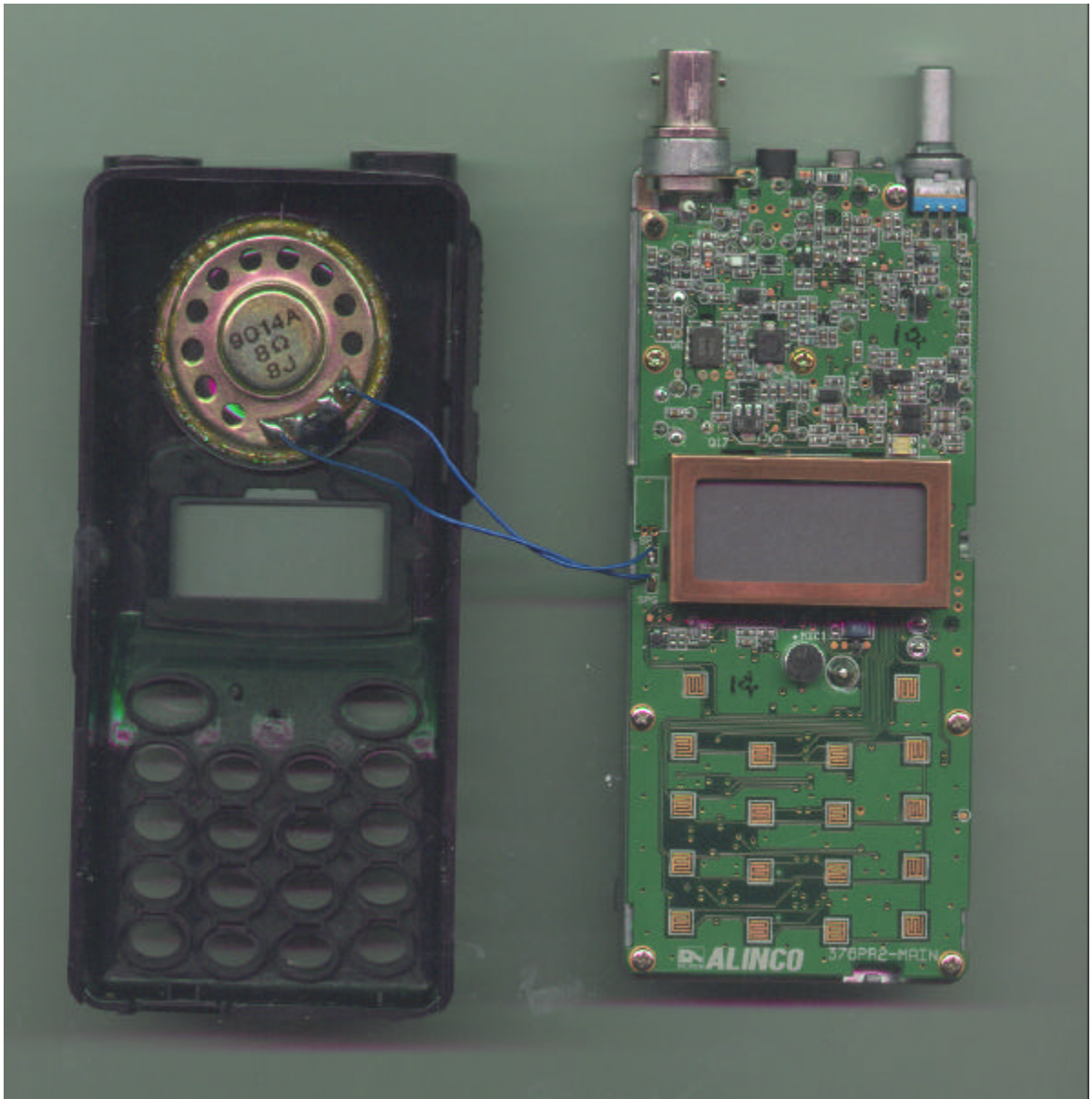
FIGURE 3: EUT without Cover
