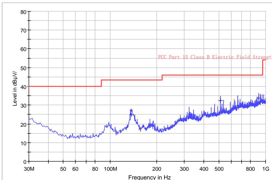
Graphic 1 Radiated Emissions
