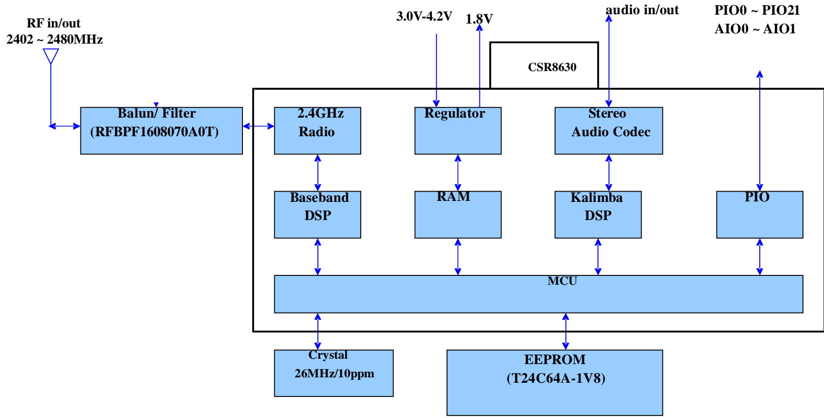
Block Diagram
