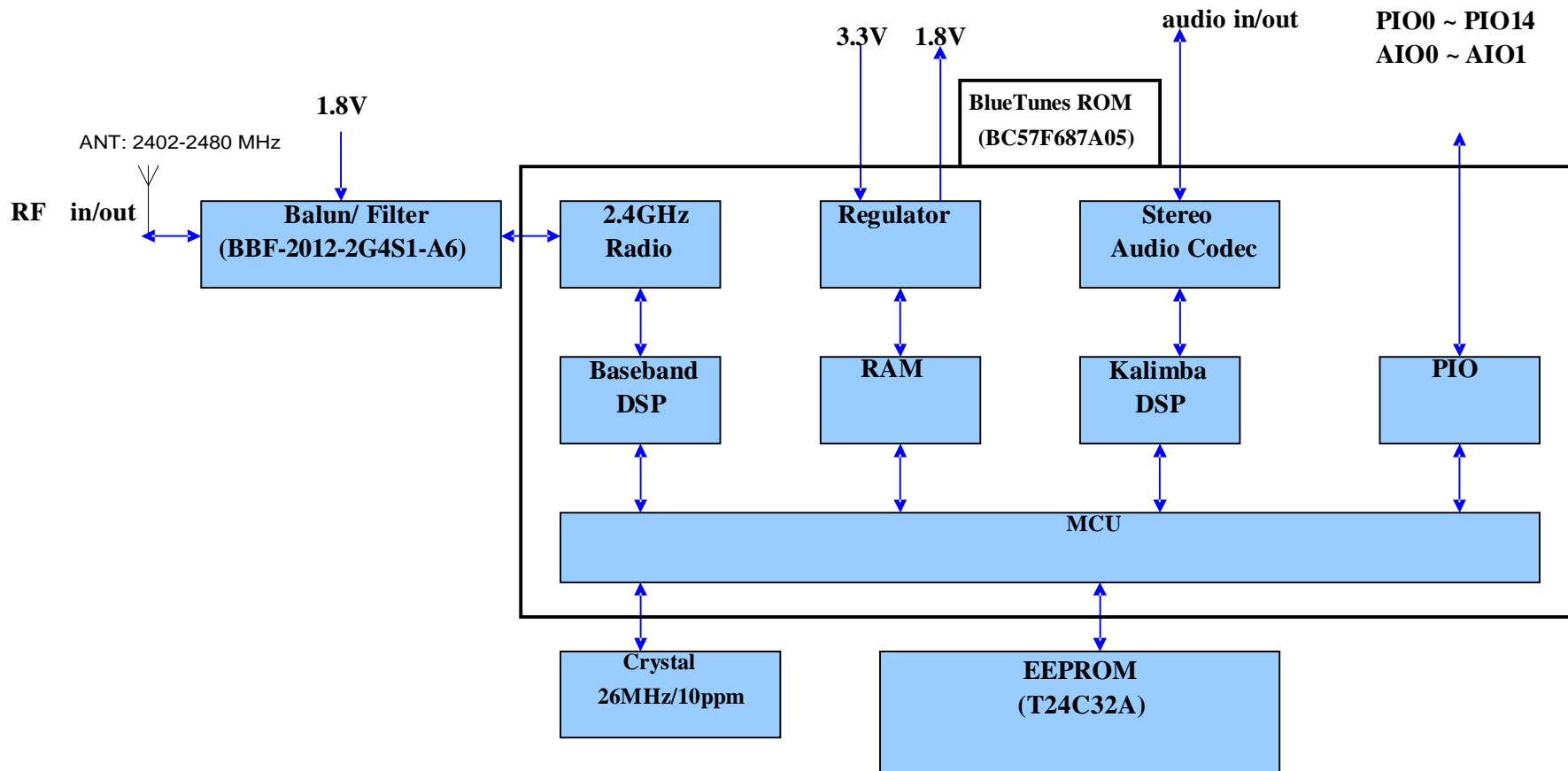
JS-BTM521 Block Diagram
