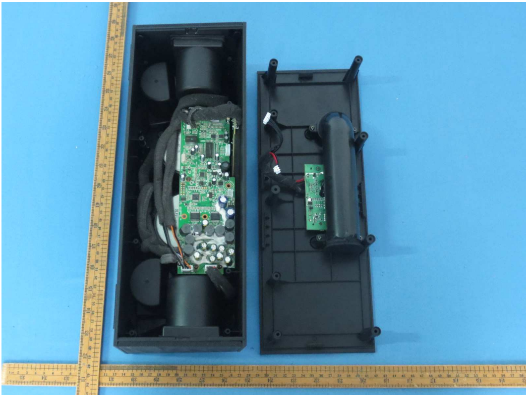
Internal photos
