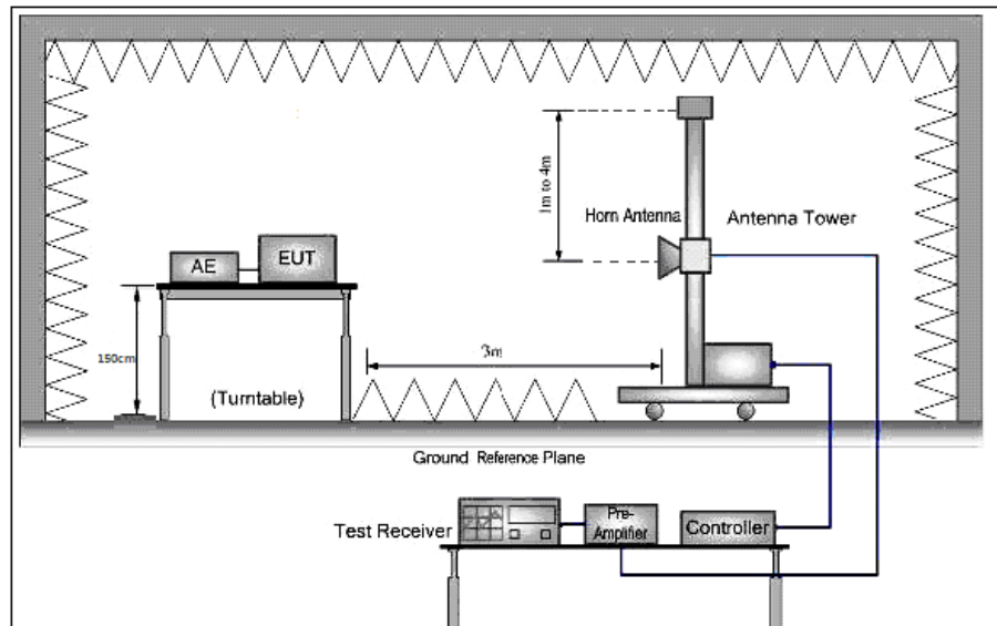
Figure 3. Above 1 GHz
