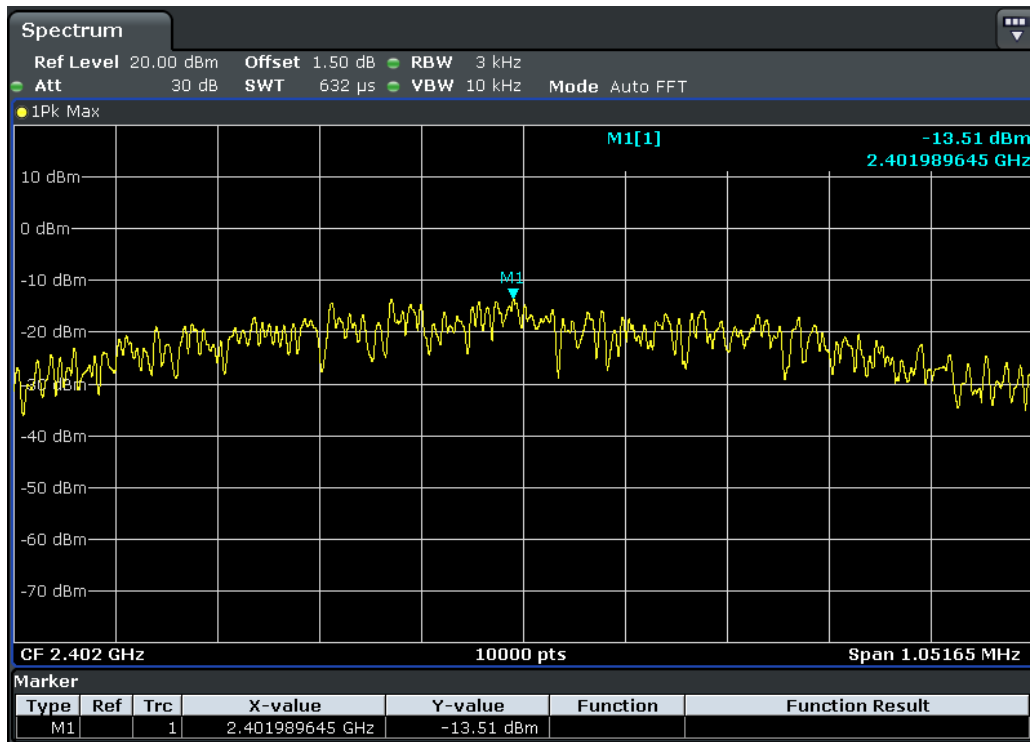
PSD 3kHz (1Mbps) The Lowest Channel 00: 2402MHz
