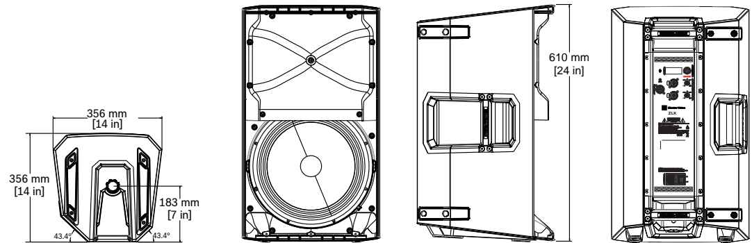
Figure 7.1: Dimensions ZLX-12BT
