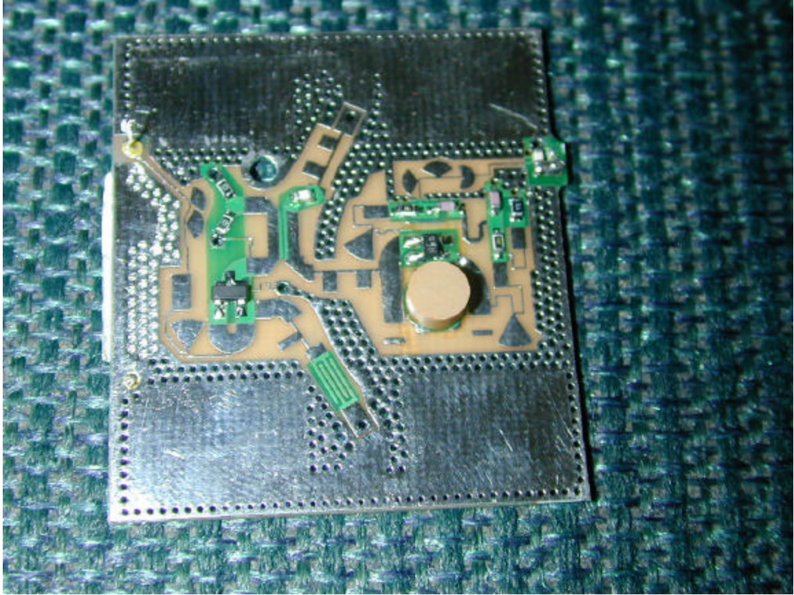
PCB with tuning cover removed
