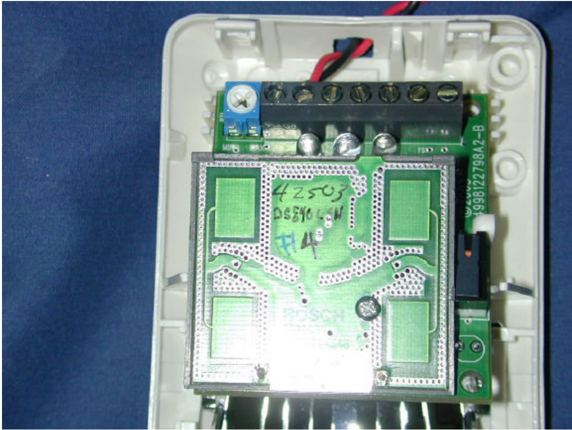
PCB Mounted in Chassis
