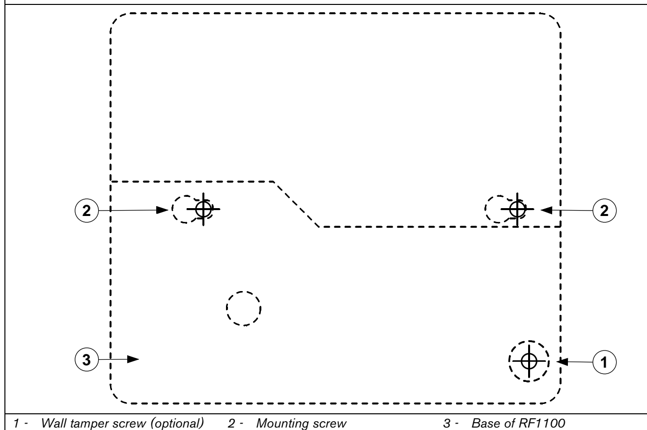
Figure 1: RF1100 Mounting Template (Actual size)
