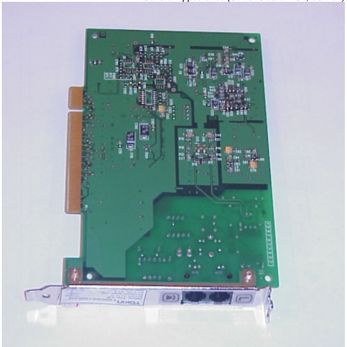
Photos 3 General Appearance (Solder Side of EUT, I/O Port)
