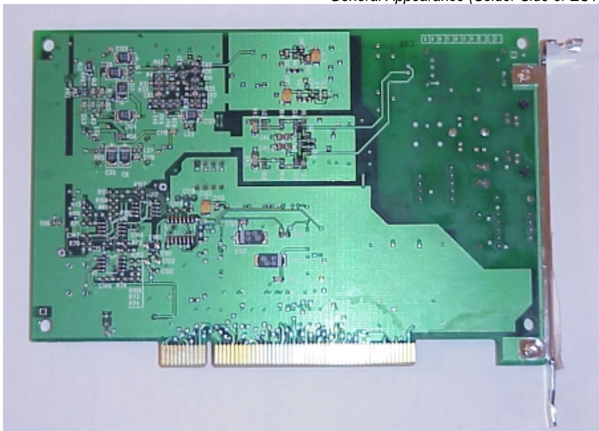
Photos 2 General Appearance (Solder Side of EUT)
