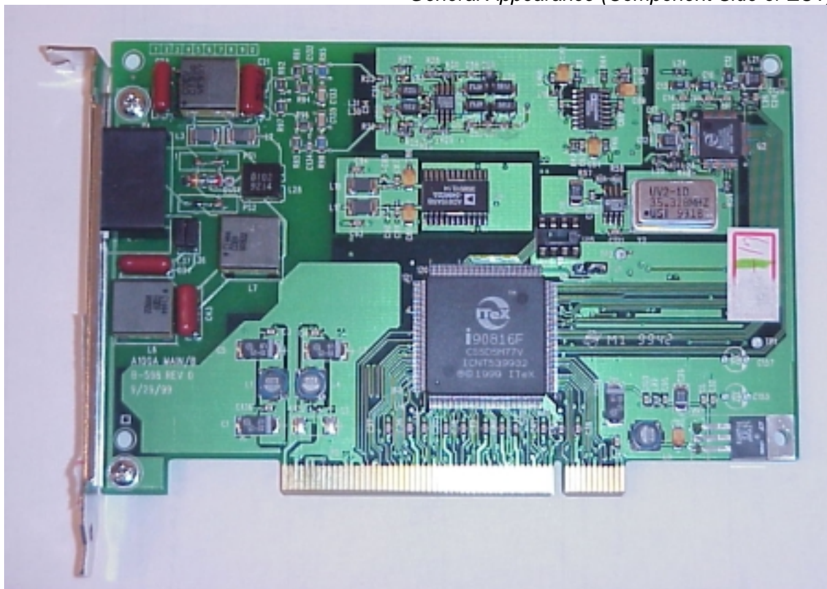
Photos 1 General Appearance (Component Side of EUT)
