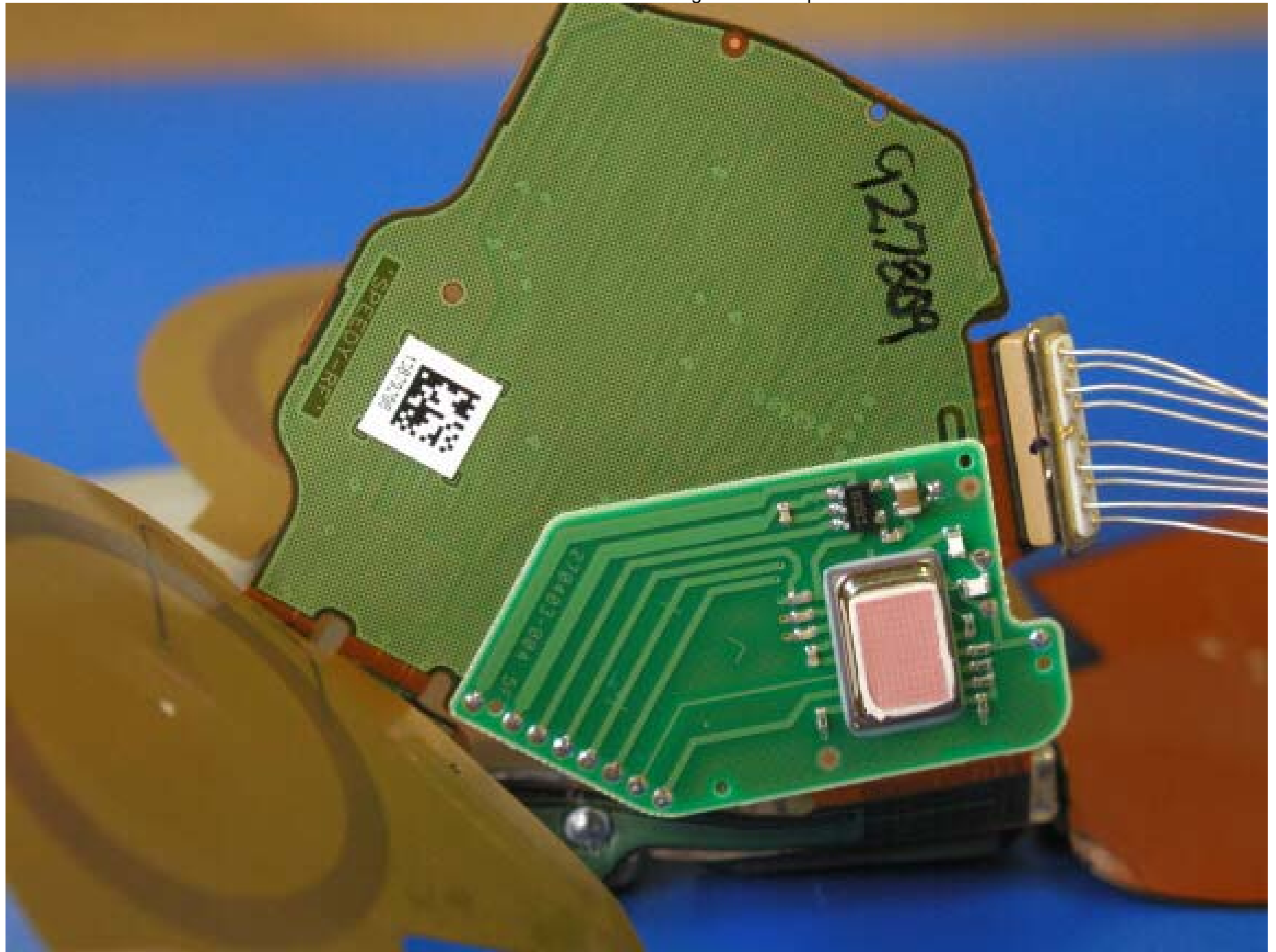
Motherboard - Back and Daughterboard Top
