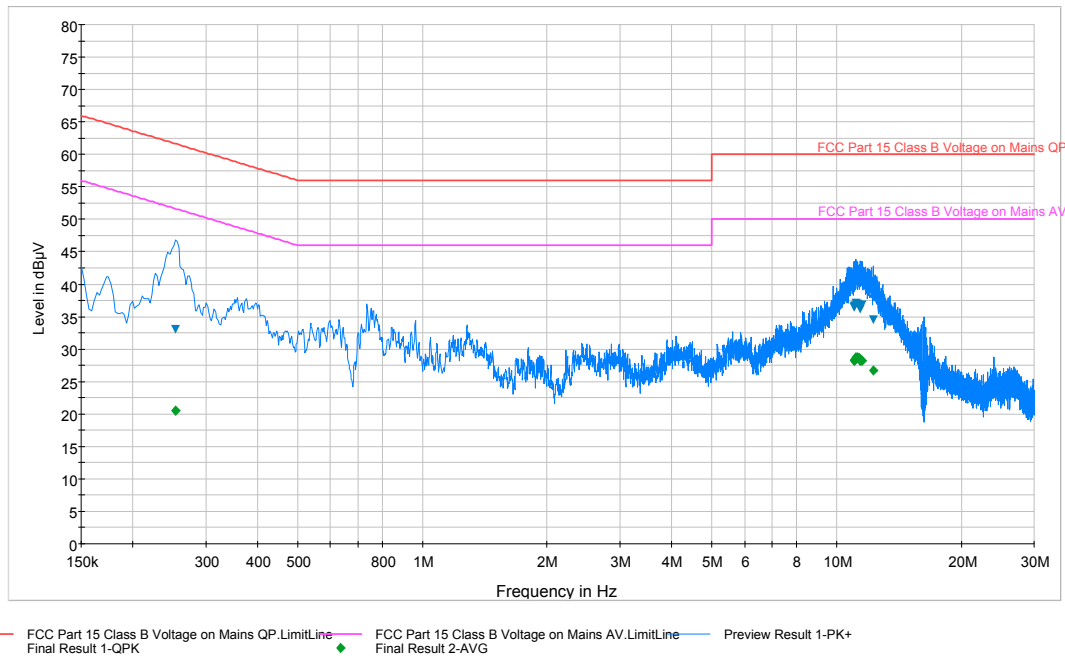
Plot 6-10. Line-Conducted Test Plot (L1)
