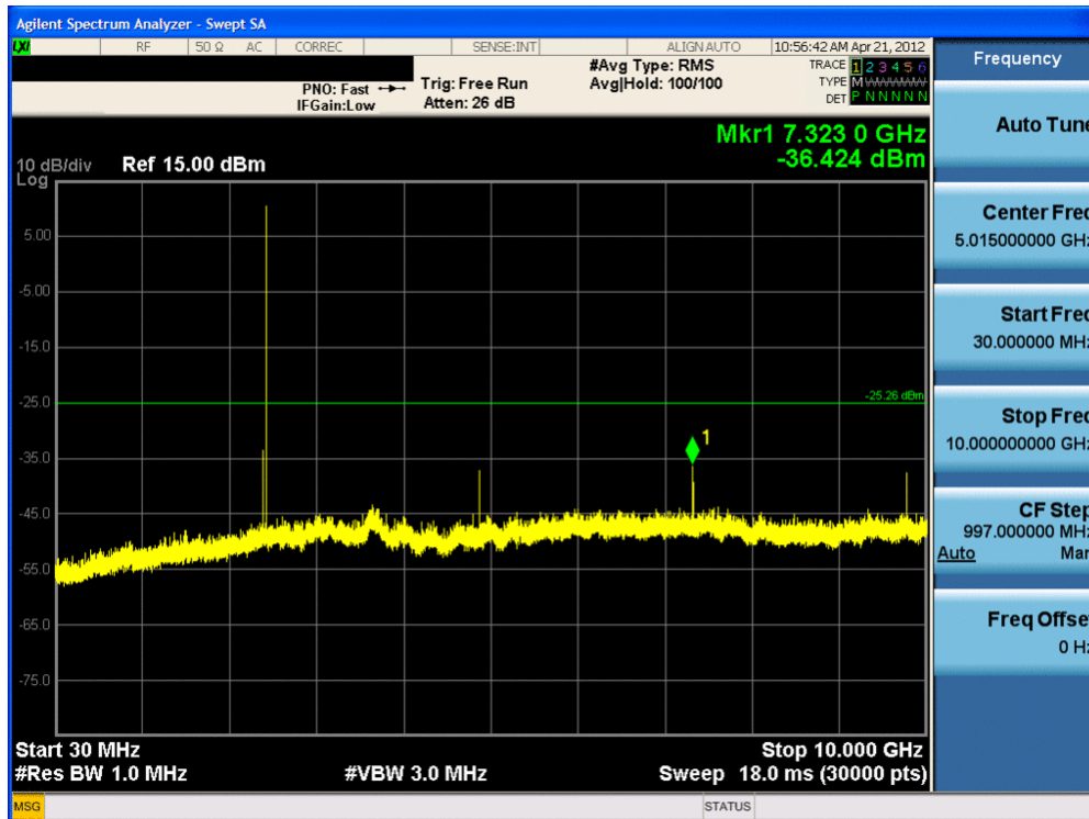
Plot 6-20. Conducted Spurious Plot (Bluetooth, 2Mbps – Ch. 39)
