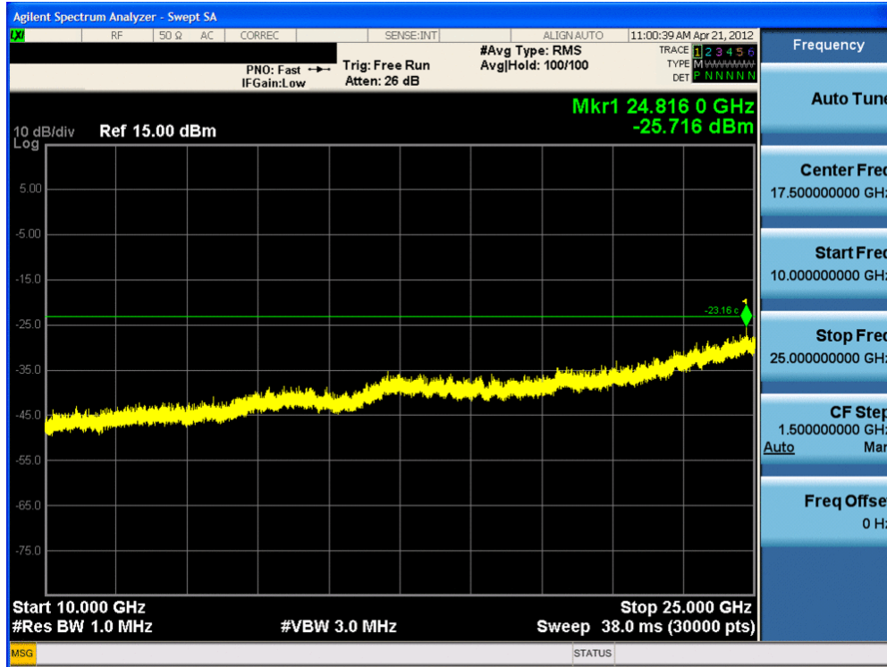
Plot 6-19. Conducted Spurious Plot (Bluetooth, 2Mbps – Ch. 0)
