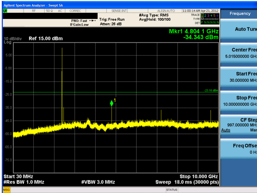
Plot 6-18. Conducted Spurious Plot (Bluetooth, 2Mbps – Ch. 0)
