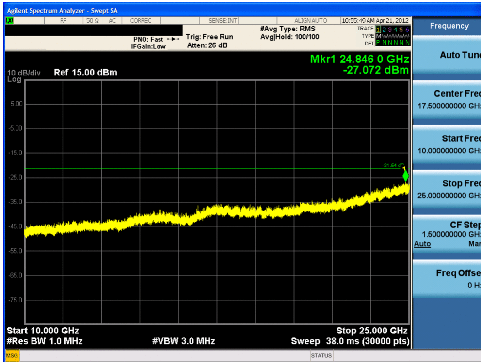
Plot 6-23. Conducted Spurious Plot (Bluetooth, 2Mbps – Ch. 78)
