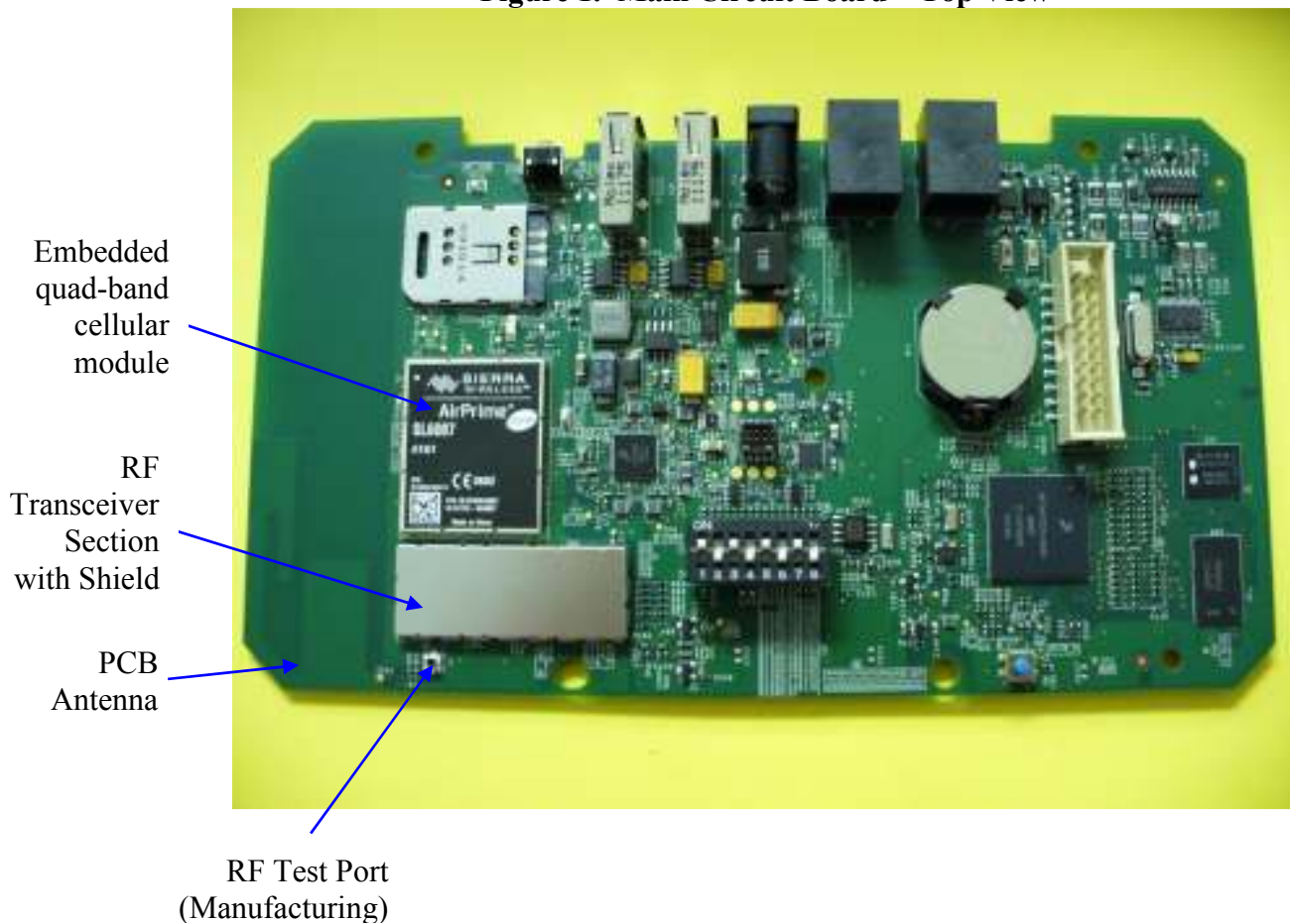
Figure 1. Main Circuit Board – Top View
