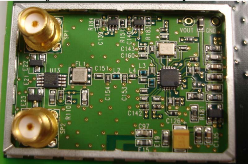
Figure 2. Transceiver Section – Top View
