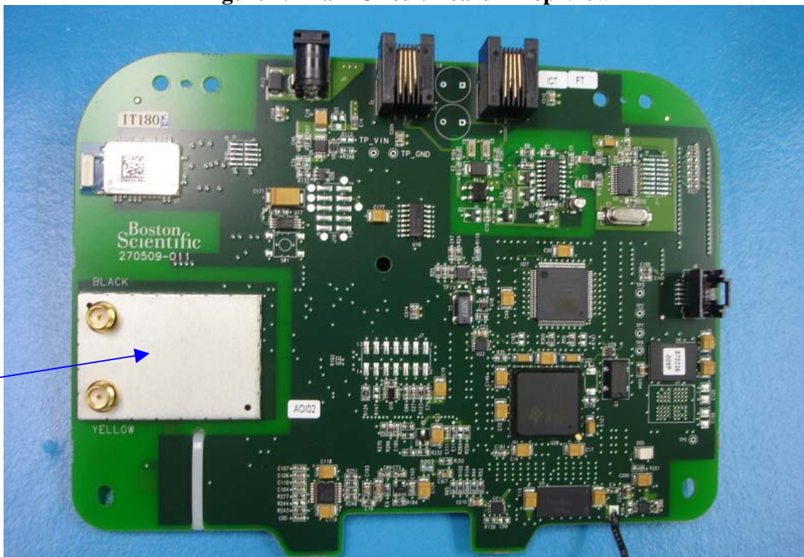
Figure 1. Main Circuit Board – Top View
