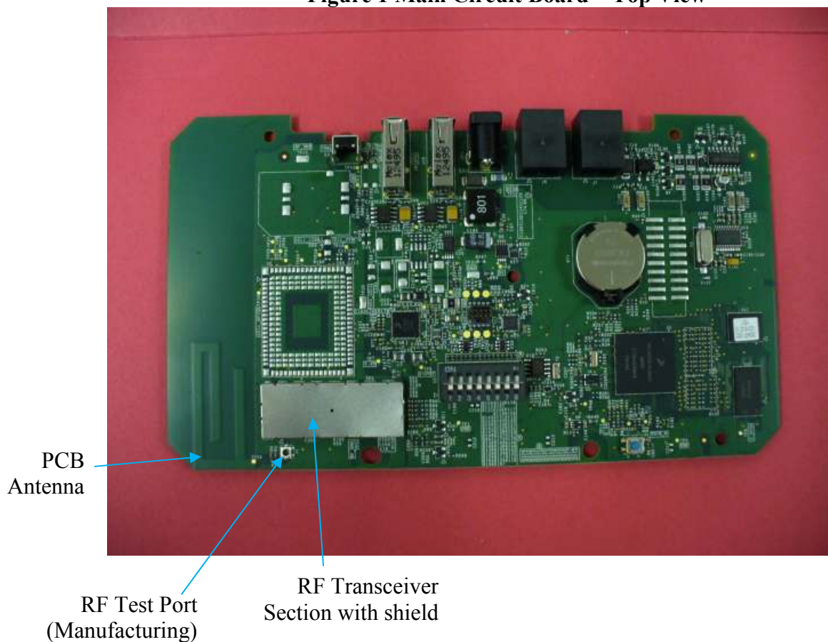
Figure 1 Main Circuit Board – Top View
