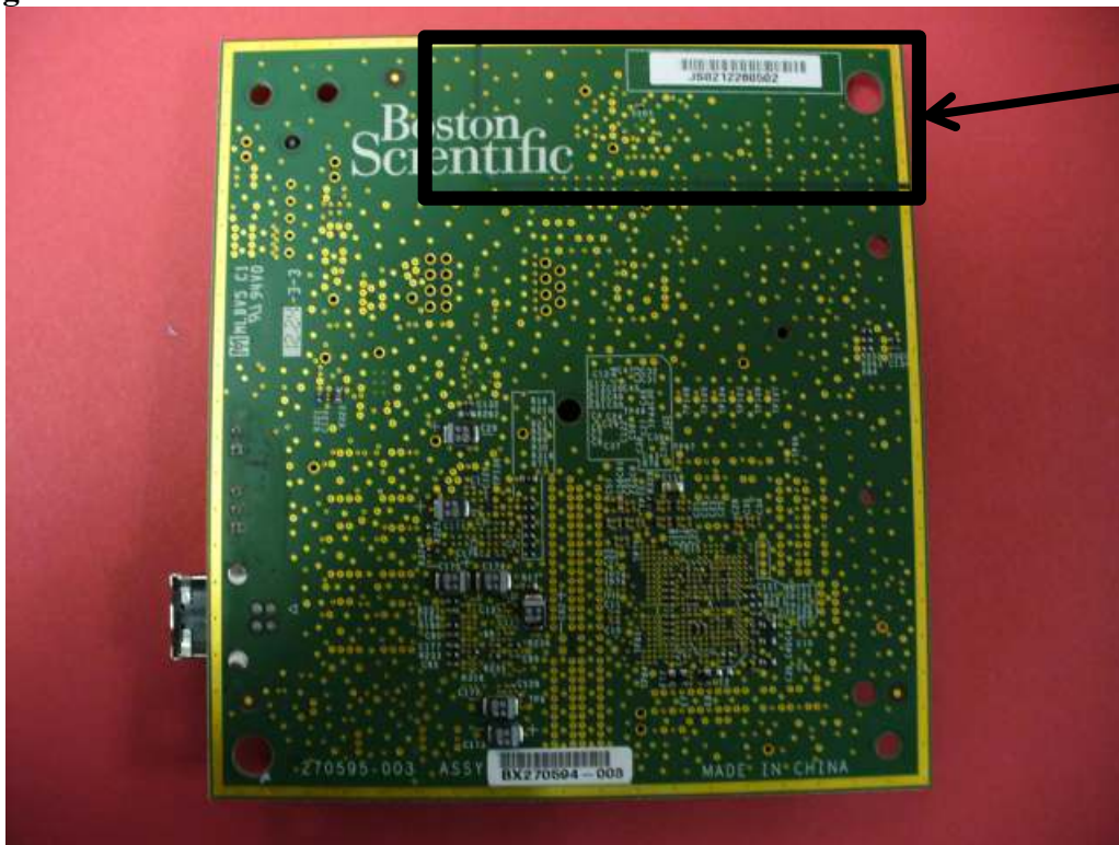
Figure 3 Model 3140 Zoom Wireless Transmitter – Control Board Bottom View
