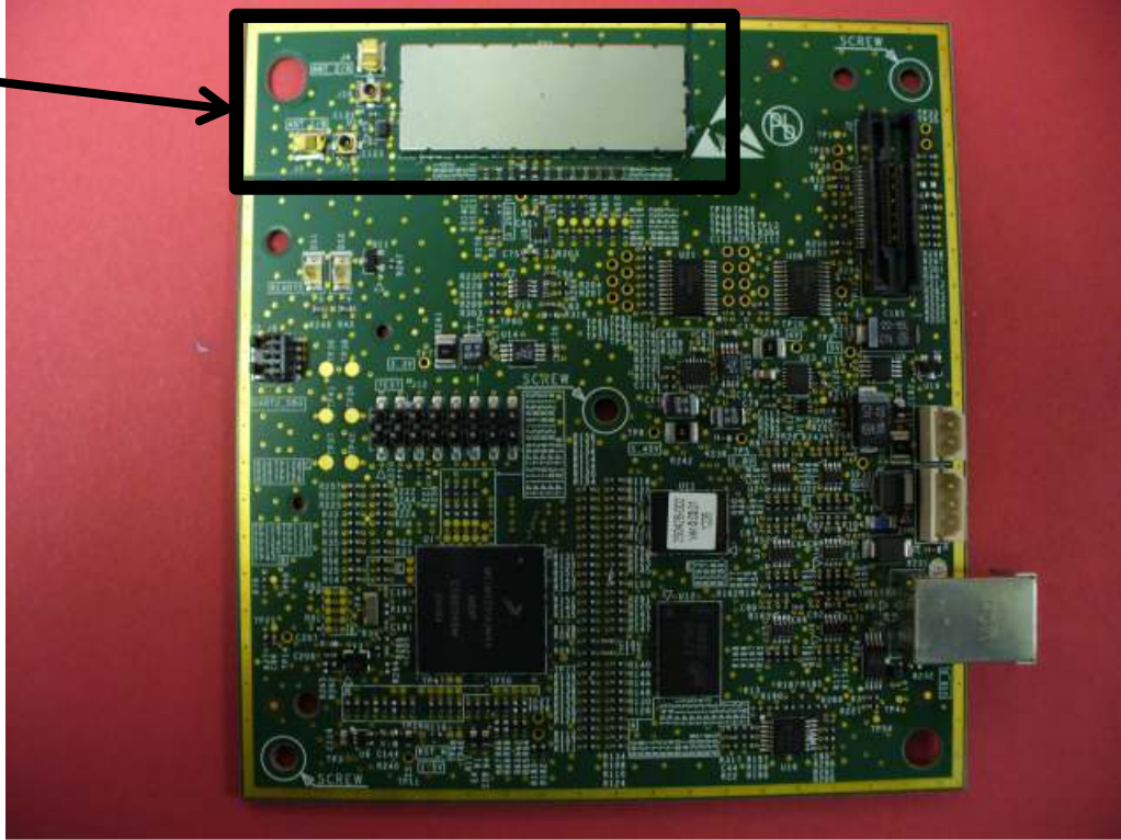
Figure 2 Model 3140 Zoom Wireless Transmitter – Control Board Top View
