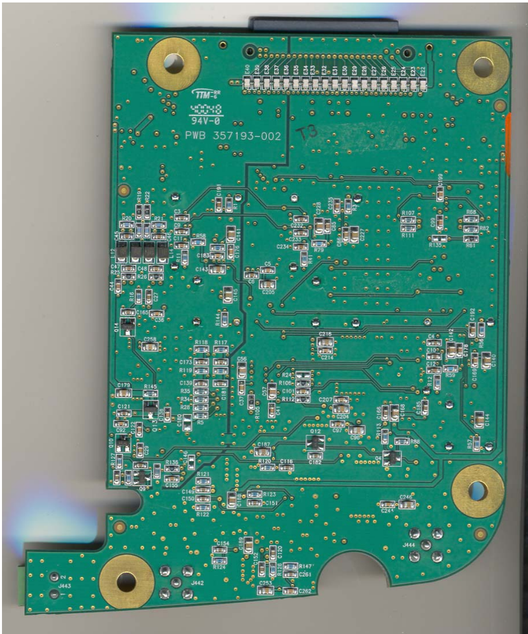
RF Analog Board Back
