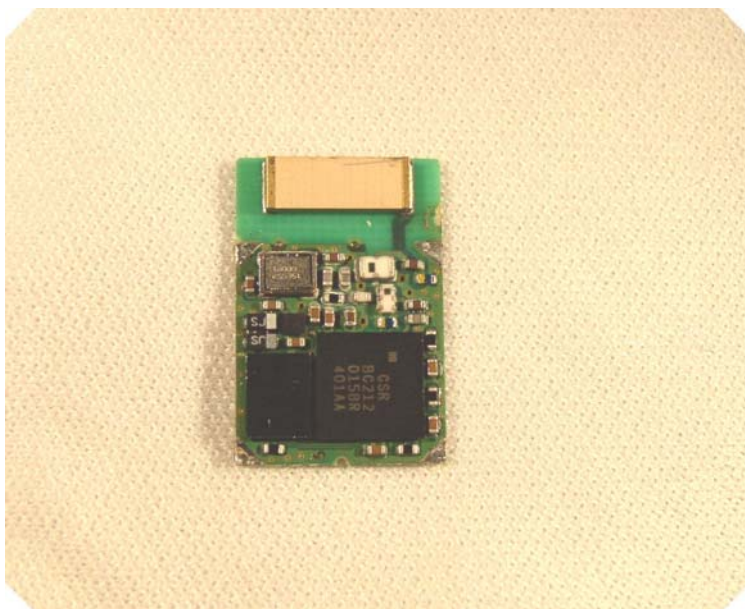
Figure 2: Photo of Bluetooth Radio without PCB shield:
