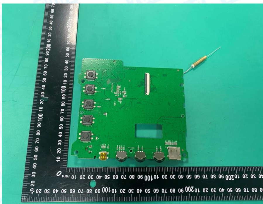
Photo 15 Appearance of PCB
