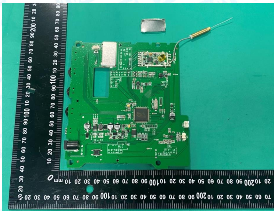
Photo 17 Appearance of PCB
